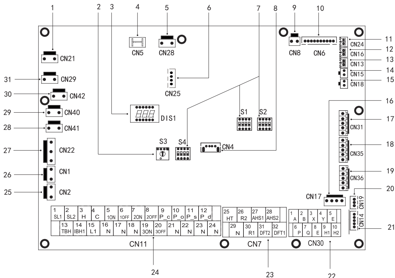
fig. 22 - Hydronic board
